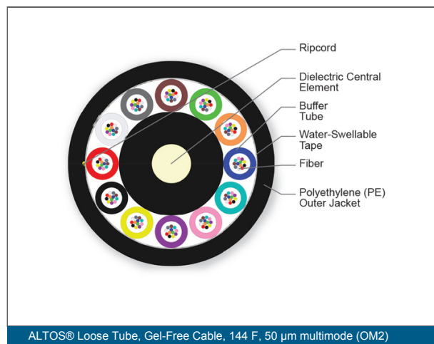
ALTOS® Loose Tube, Gel-Free Cable, 144 F, 50 µm multimode (OM2)
